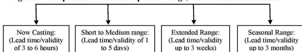
Figure 9: Temperature Forecast
