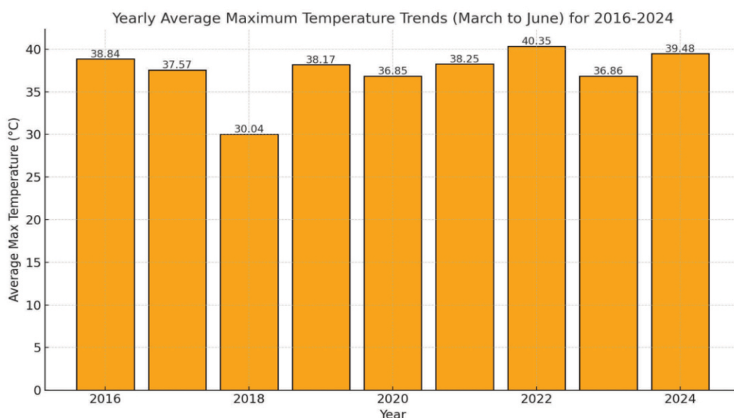
Figure 3: Yearly average Maximum temperature trends (March to June) for the last decade (2016-2024)
