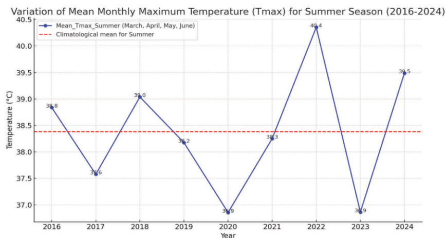
Figure A2: Variation of average monthly Tmax for summer months
