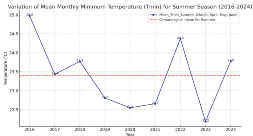
Figure A4: Variation of average monthly Tmin for summer months
