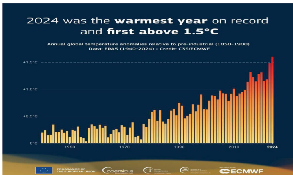
Figure 1: Annual global Temperature anomalies relative to pre-industrial (1850-1900) (ERAS- c3S/ECMWF)
