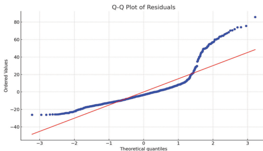
Figure A3: Q-Q plot of residuals
