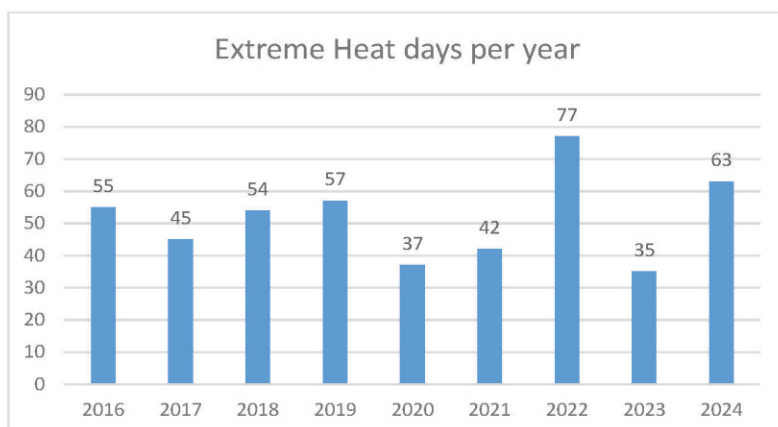
Figure 4: Trends of Extreme Heat Days (Temperature above 40°C) per years (2016-2024).
